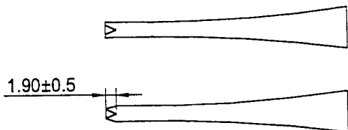
DETAIL 1 x 2 TEETH SCALE 1 : 1
