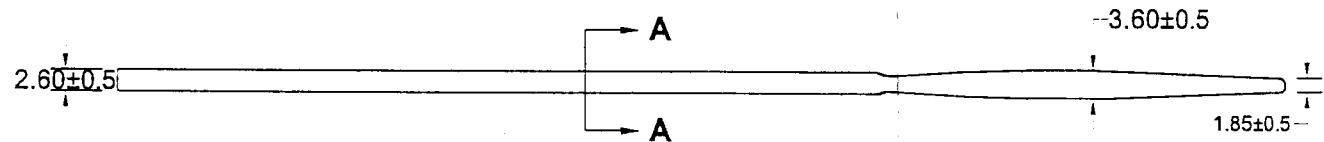
SIDE ELEVATION
